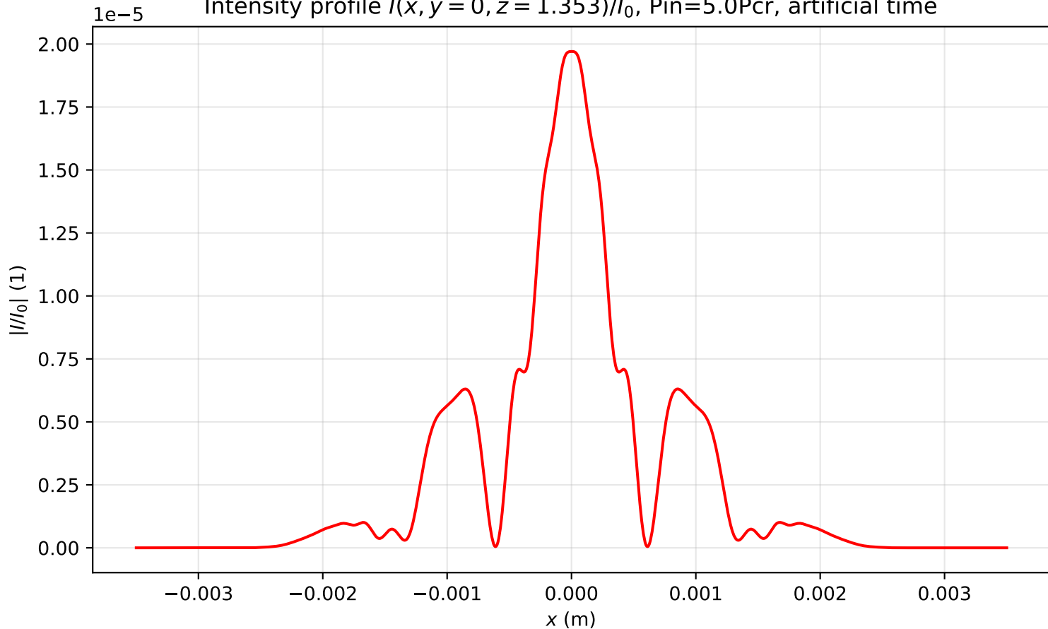
Intensity profile I(x, y = 0, z = 1.353)/I_0 , P_{in}=5.0P_{cr} , artificial time
